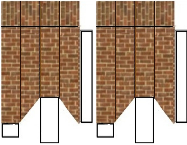
End roof support sections for main house
